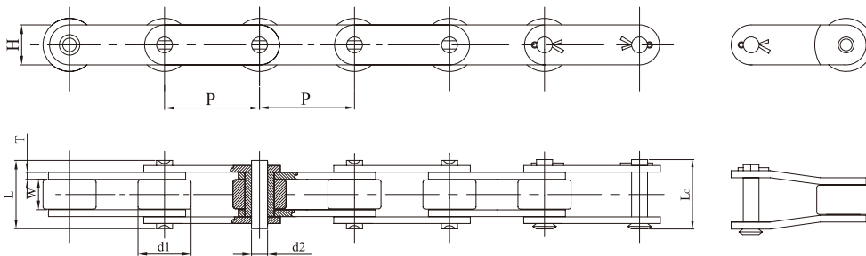
Roller chain with big rollers
